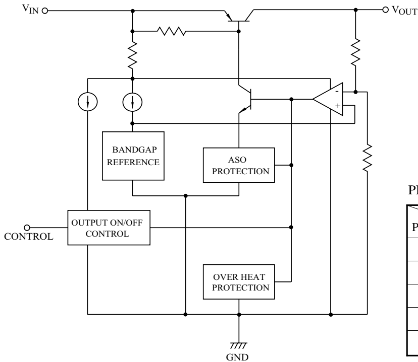
BLOCK DIAGRAM - 2 (Fixed-Type)
