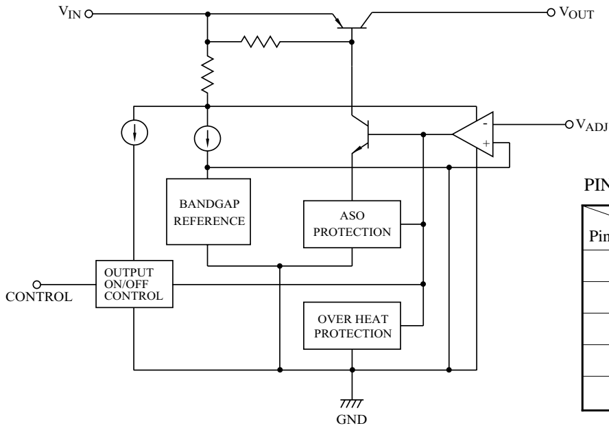
BLOCK DIAGRAM - 1 (Adjustable-Type)
