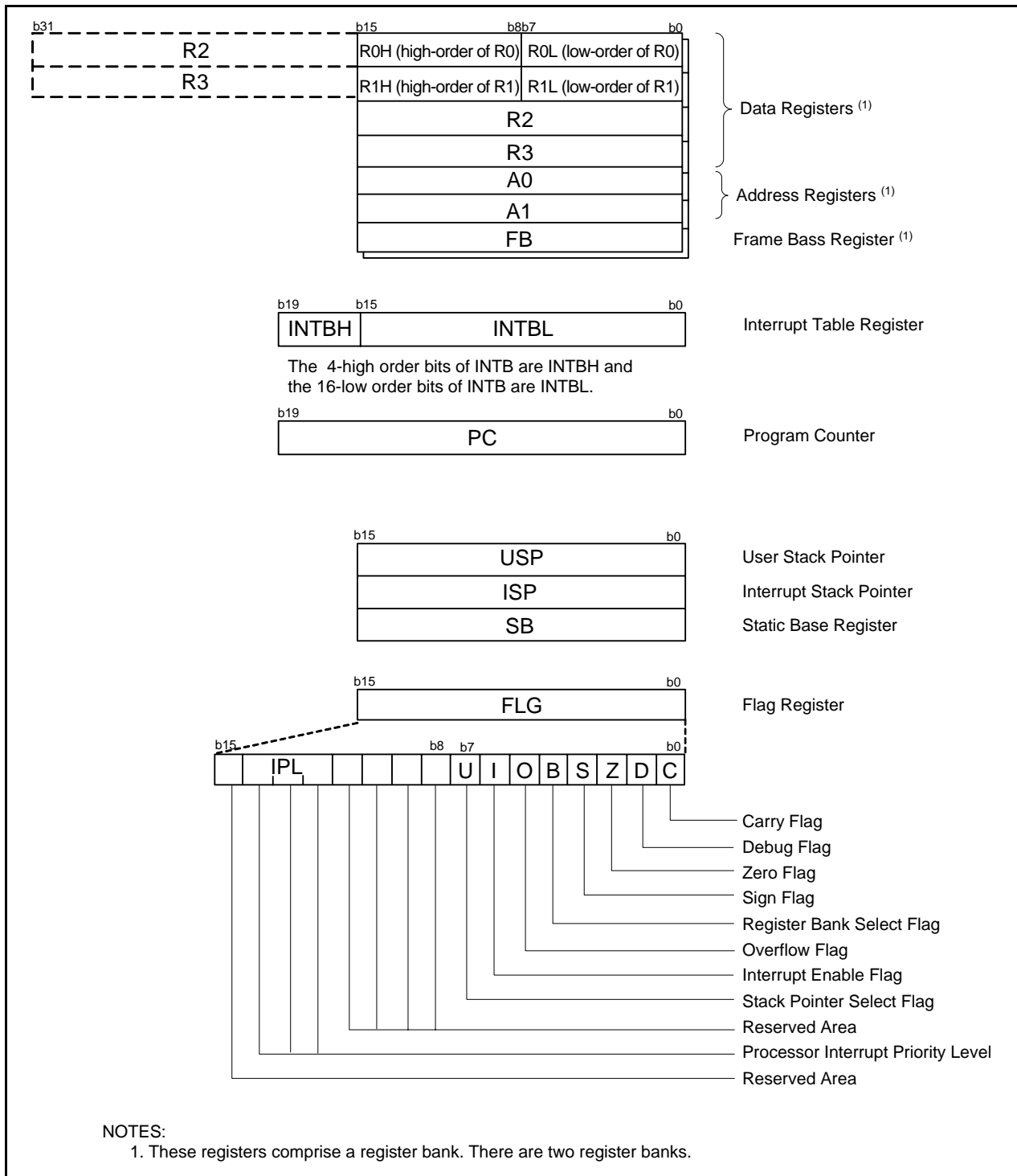
Figure 2.1 CPU Register
