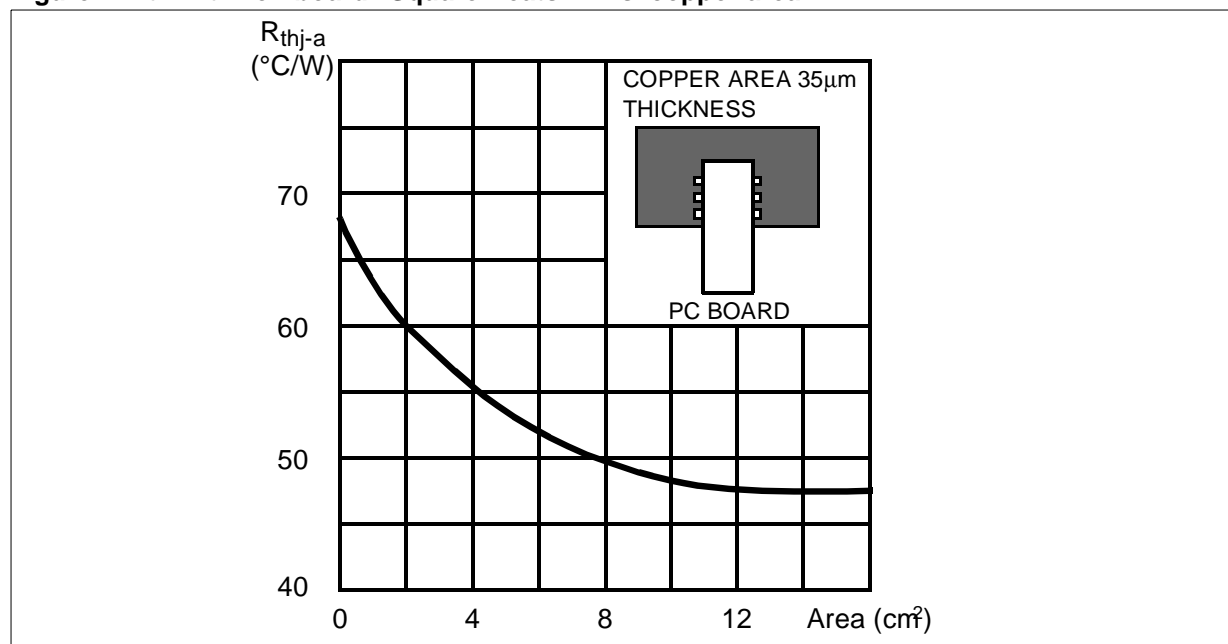
Figure 2. R thj-a with “on board” Square Heatsink vs. copper area
