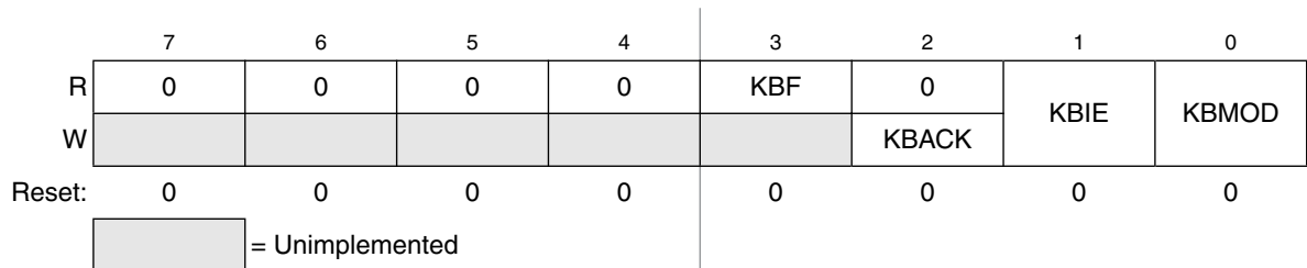
Figure 12-3. KBI Status and Control Register
