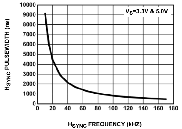
FIGURE 2. H_{SYNC} PULSEWIDTH vs H_{SYNC} FREQUENCY ( R_{SET} = OPEN )
