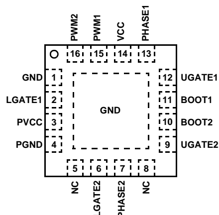
ISL6614BCR/ISL6614BCRZ (16 LEAD QFN) TOP VIEW
