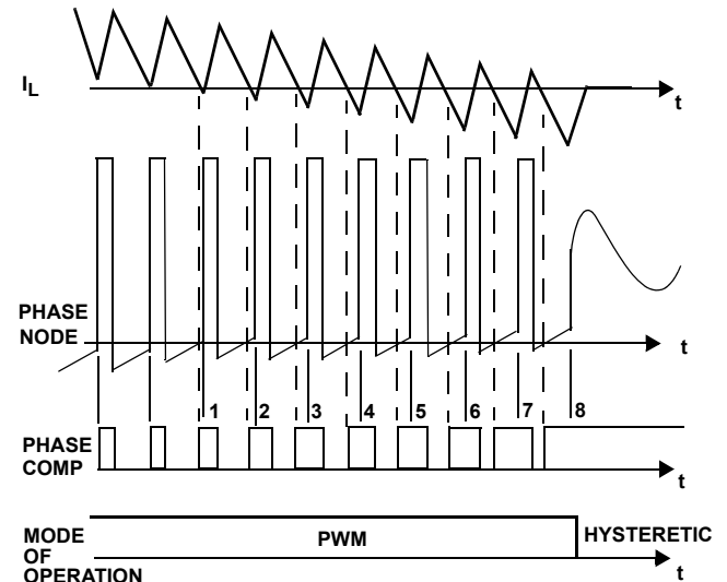
FIGURE 3. MODE CONTROL WAVEFORMS
