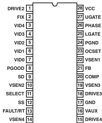
ISL6440A (SOIC) TOP VIEW
