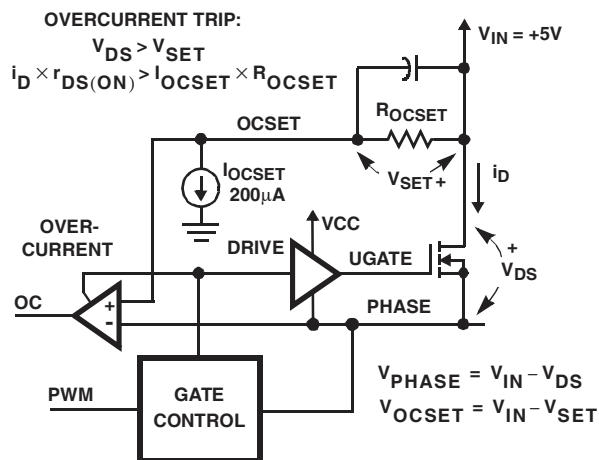
FIGURE 5. OVERCURRENT DETECTION
