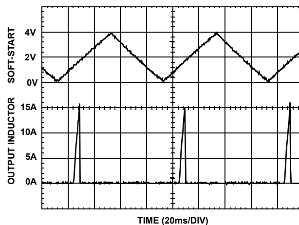
FIGURE 4. OVERCURRENT OPERATION
