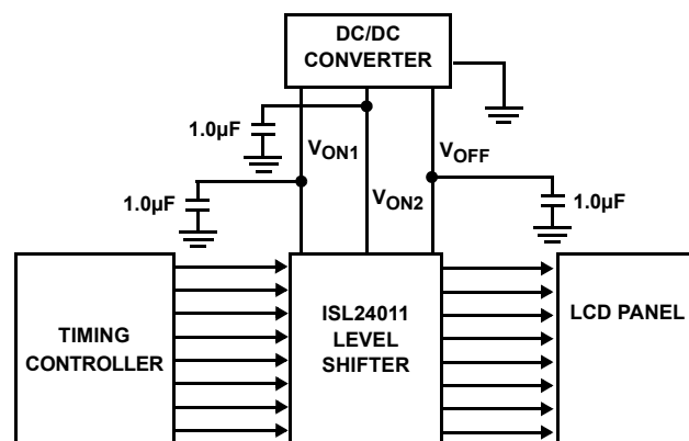
FIGURE 14. TYPICAL TV APPLICATION CIRCUIT
