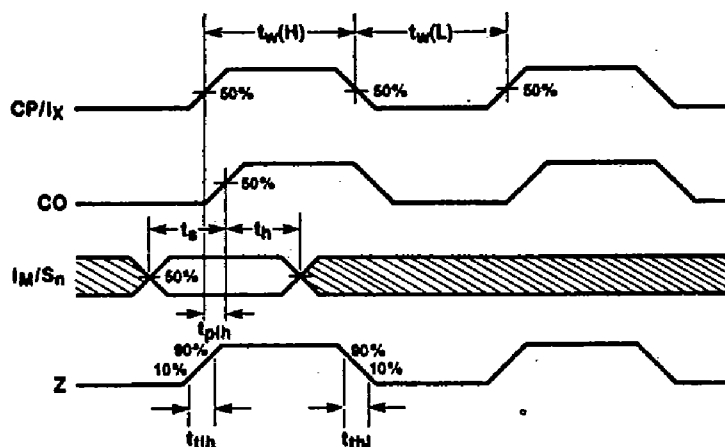
Figure 3: Switching Waveforms
