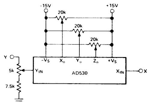
Figure 2. Adjustment Pot Connections (Multiplier Mode)
