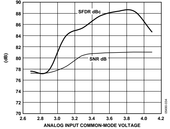
Figure 34. AD9446-80 SNR/SFDR vs. Analog Input Common Mode, 80 MSPS
