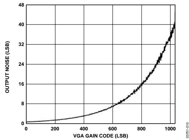
Figure 9. Output Noise vs. VGA Gain
