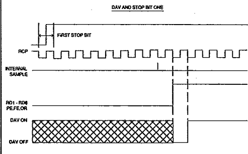
FIG. 8 RECEIVER DURING 1ST STOP BIT
