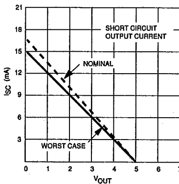
FIG. 19 SHORT CIRCUIT OUTPUT CURRENT (only 1 output may be shorted at a
