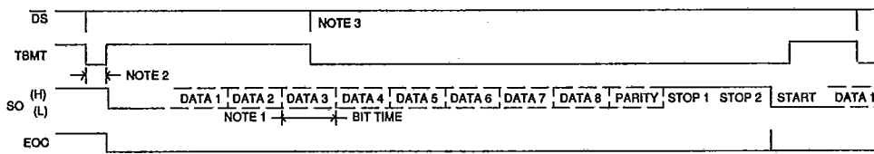
FIG. 1 UAR/T - TRANSMITTER TIMING
