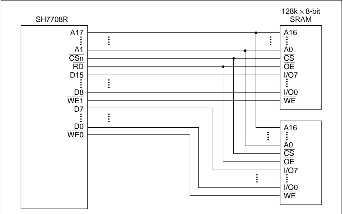
Figure 10.8 Example of 16-Bit Data Width SRAM Connection
