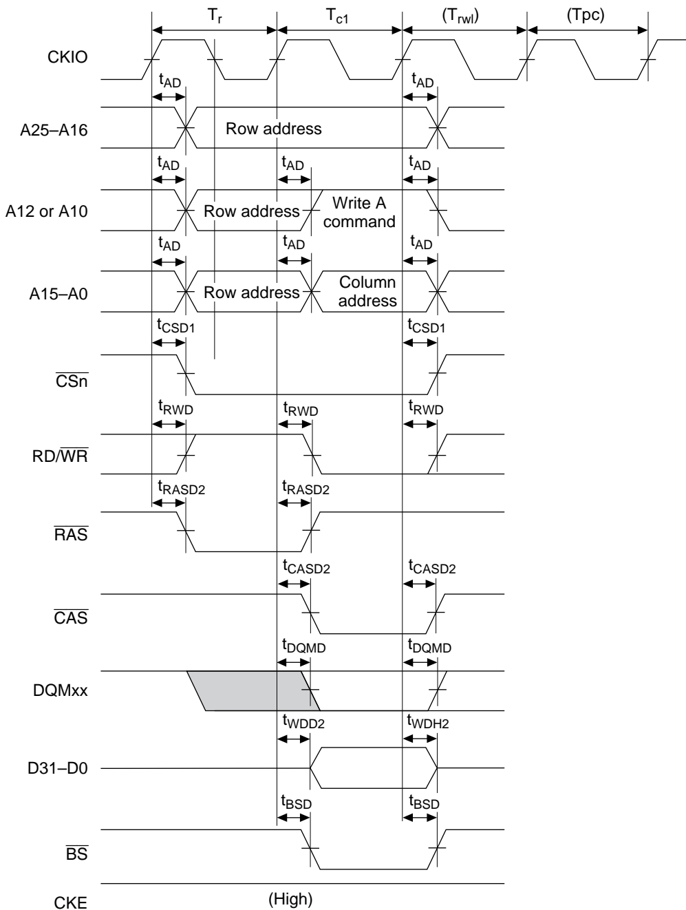
Figure 16.38 Synchronous DRAM Write Bus Cycle (RCD = 0, TPC = 0, TRWL = 0)
