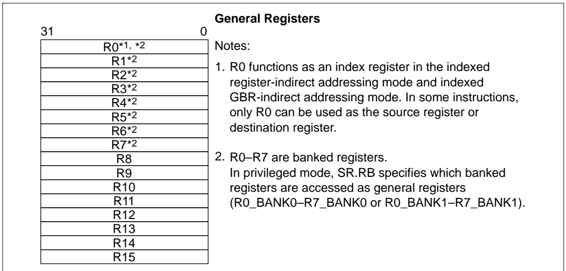
Figure 2.3 General Registers
