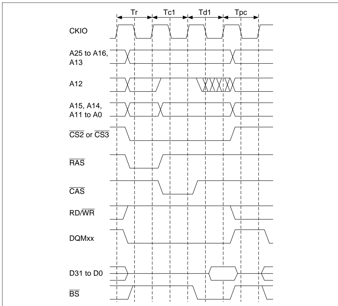
Figure 10.26 Basic Timing for Synchronous DRAM Single Read
