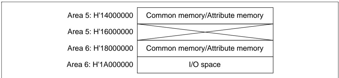
Figure 10.4 PCMCIA Space Allocation
