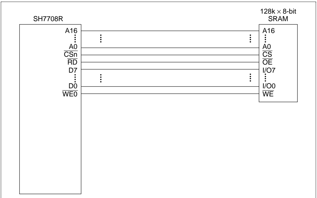
Figure 10.9 Example of 8-Bit Data Width SRAM Connection
