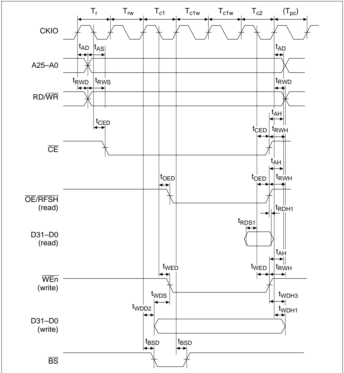
Figure 17.46 Pseudo-SRAM Read Cycle (RCD = 1, A3W = 3, TPC = 0)
