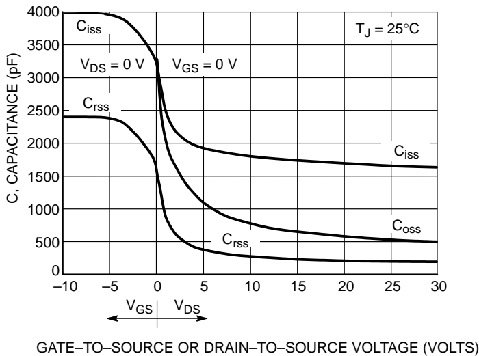
Figure 7. Capacitance Variation
