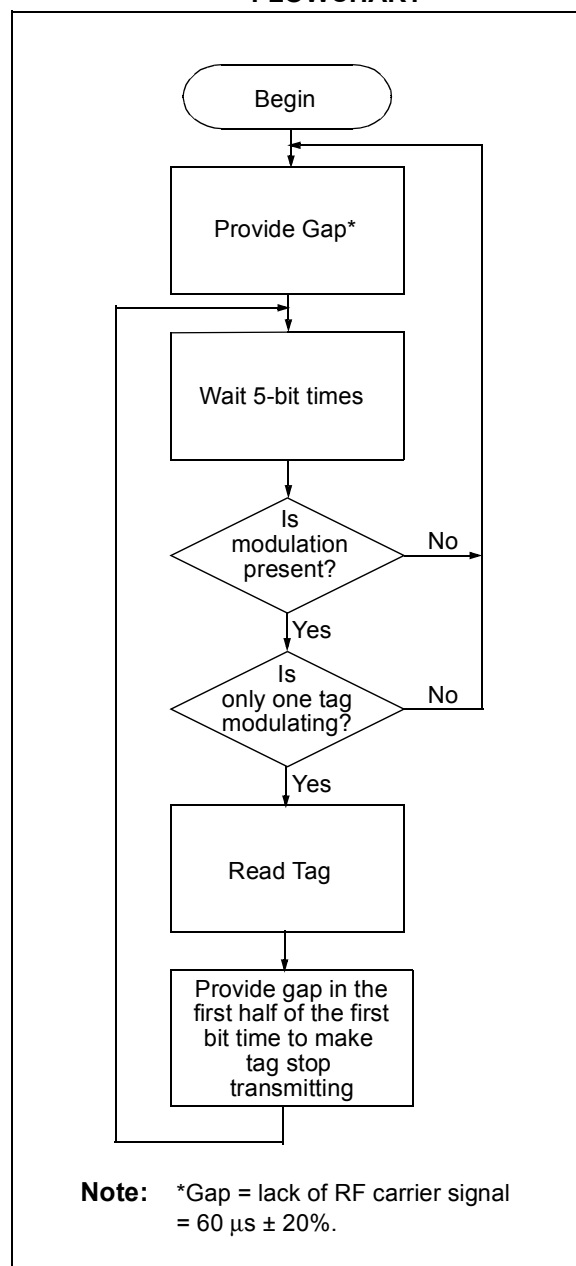
FIGURE 5-1: ANTI-COLLISION FLOWCHART
