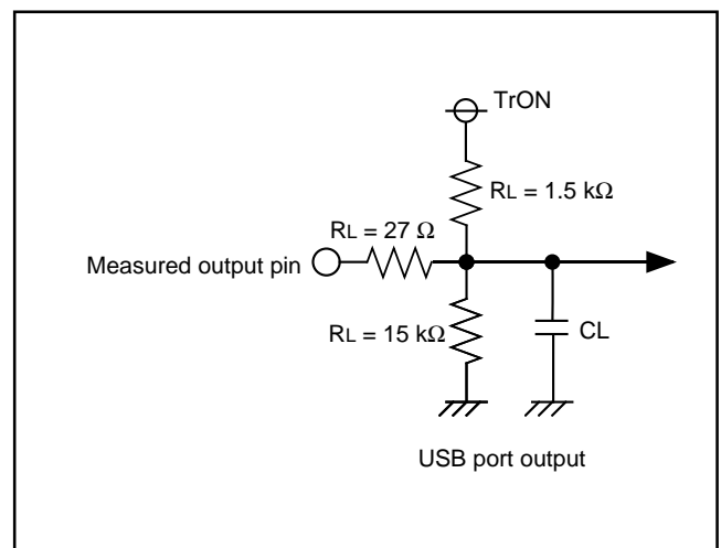
Fig. 173 USB output switching characteristics measurement circuit (2) for D0+, D1+/D2+ (full-speed), D1-/D2- (low-speed)
