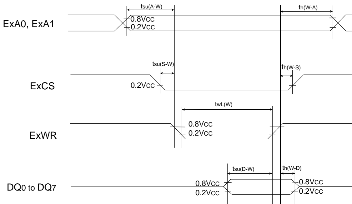
Fig. 175 Timing chart (2)
