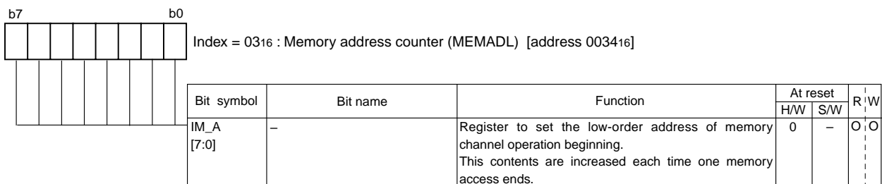
Fig. 118 Index03[low]; Structure of Memory address counter
