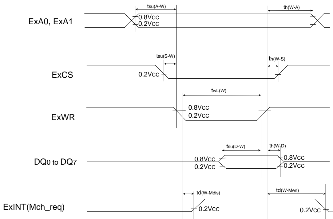
Fig. 176 Timing chart (3)
