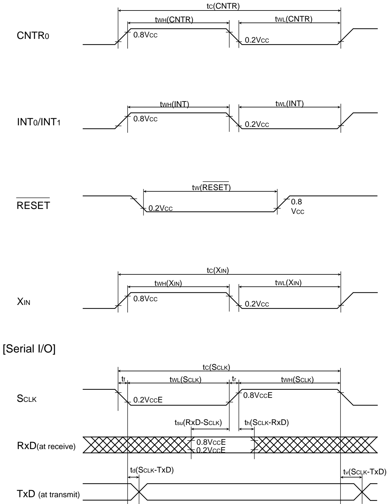
Fig. 174 Timing chart (1)
