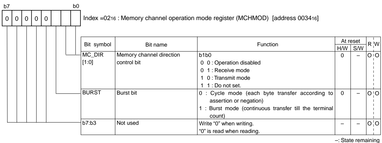
Fig. 117 Index02[low]; Structure of Memory channel operation mode register
