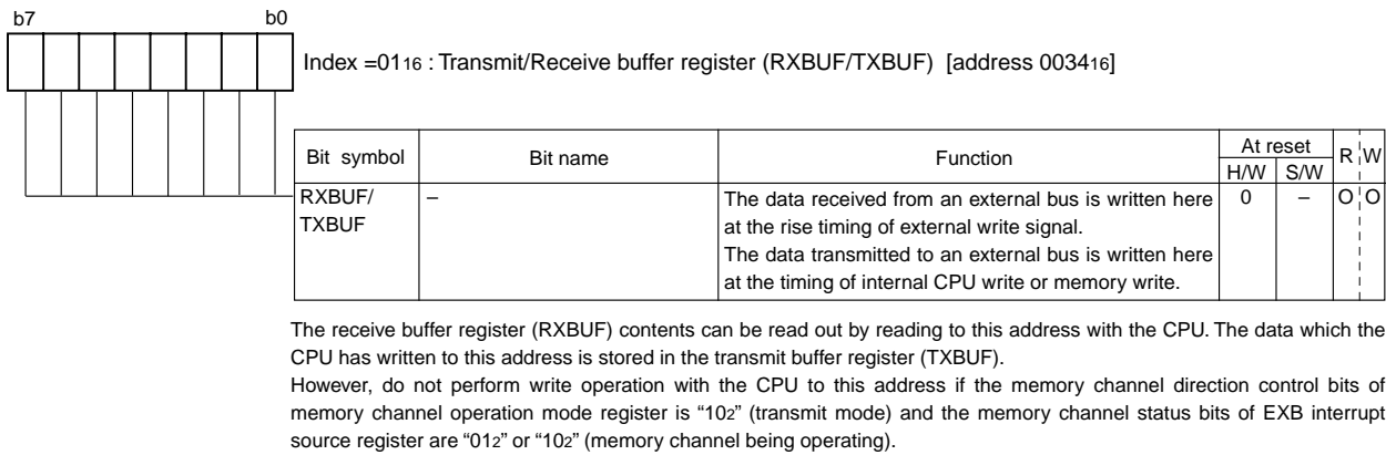
Fig. 116 Index01[low]; Structure of Transmit/Receive buffer register
