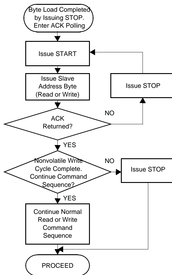
FIGURE 9. ACKNOWLEDGE POLLING SEQUENCE
