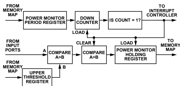
Figure 76. ADC Input Threshold Crossing Block Diagram
