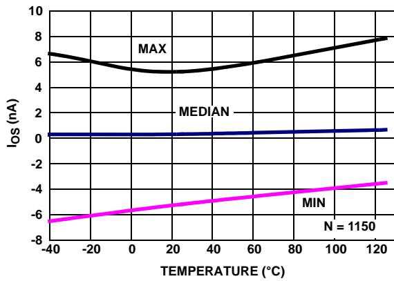
FIGURE 28. I_{OS} vs TEMPERATURE, V_+ = 5V , V_- = 0V , V_{CM} = 2.5V , R_L = \text{Open}
