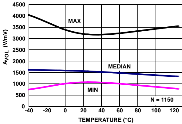
FIGURE 32. AVOL vs TEMPERATURE V_+ = 5V , V_- = 0V , V_{CM} = 2.5V , R_L = 100k
