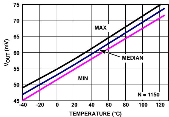
FIGURE 35. V_{OUT} LOW vs TEMPERATURE V_+ = 5V , V_- = 0V , V_{CM} = 2.5V , R_L = 1k
