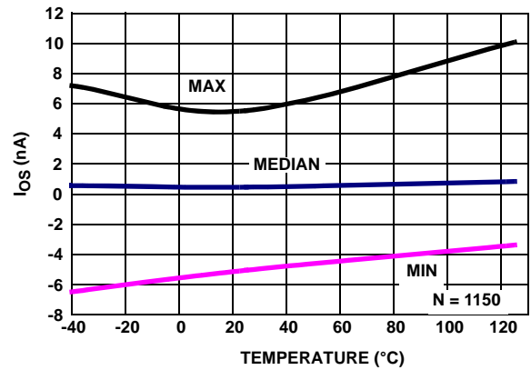
FIGURE 29. I_{OS} vs TEMPERATURE, V_+ = 5V , V_- = 0V , V_{CM} = 2.5V , R_L = \text{Open}
