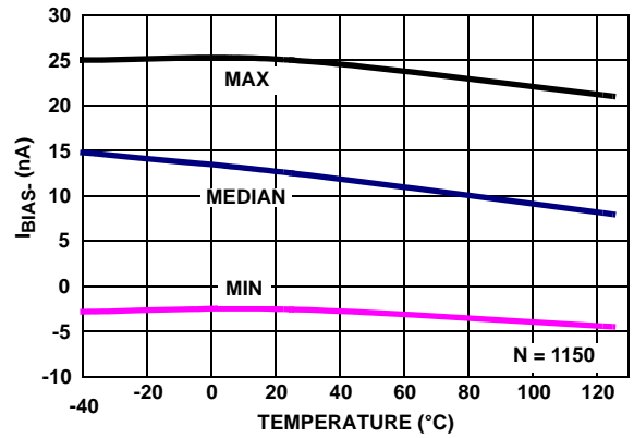
FIGURE 25. I_{BIAS-} vs TEMPERATURE, V_+ = 5V , V_- = 0V , V_{CM} = 2.5V , R_L = \text{Open}
