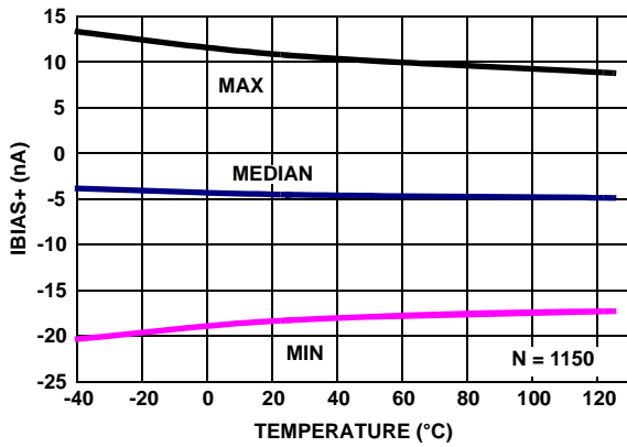
FIGURE 26. I_{BIAS+} vs TEMPERATURE, V_+ = 5V , V_- = 0V , V_{CM} = 2.5V , R_L = \text{Open}
