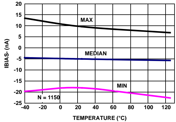
FIGURE 27. I_{BIAS-} vs TEMPERATURE, V_+ = 5V , V_- = 0V , V_{CM} = 2.5V , R_L = \text{Open}
