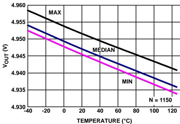
FIGURE 34. V_{OUT} HIGH vs TEMPERATURE V_+ = 5V , V_- = 0V , V_{CM} = 2.5V , R_L = 1k
