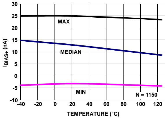
FIGURE 24. I_{BIAS+} vs TEMPERATURE, V_+ = 5V , V_- = 0V , V_{CM} = 2.5V , R_L = \text{Open}
