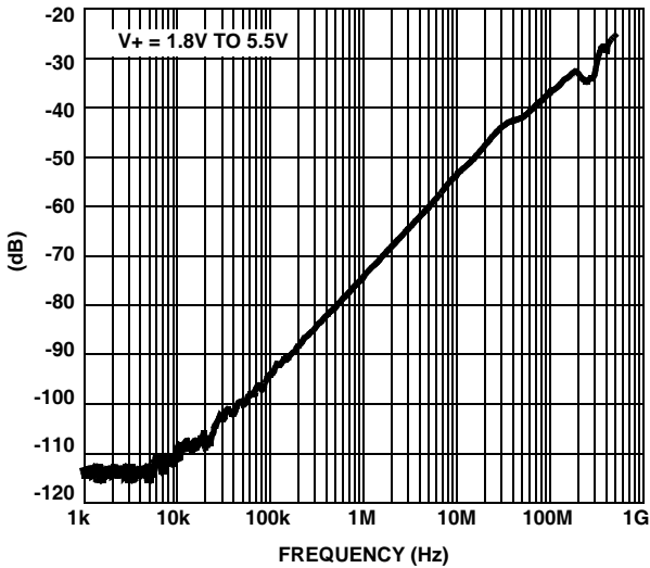
FIGURE 18. OFF ISOLATION
