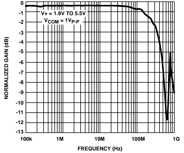
FIGURE 17. FREQUENCY RESPONSE
