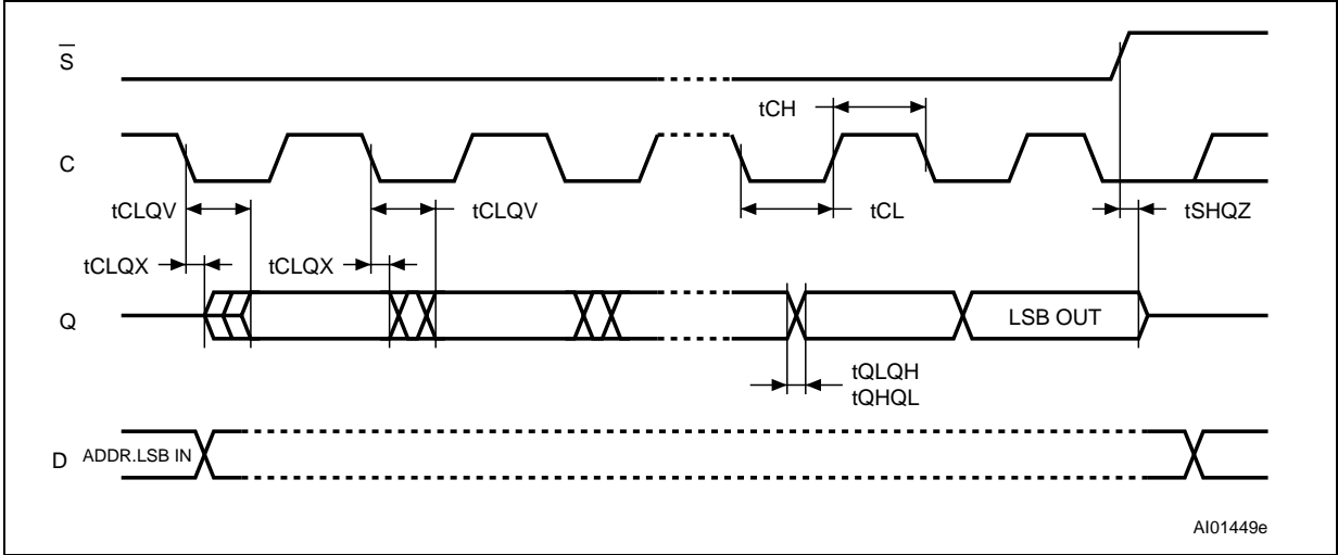
Figure 28. Output timing
