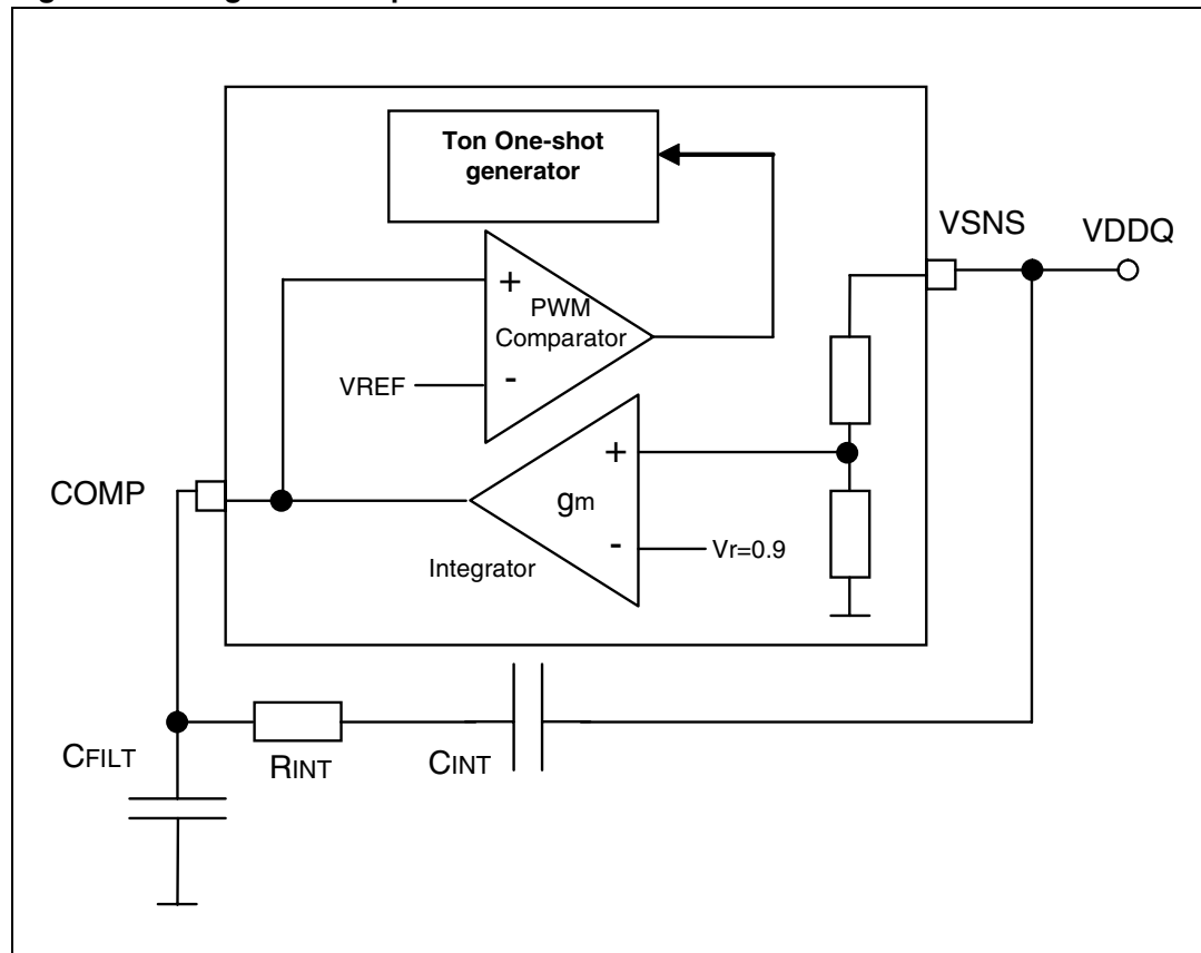
Figure 42. Integrative compensation
