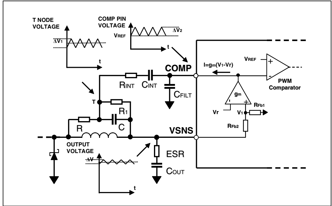
Figure 32. "Virtual-ESR" Network
