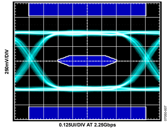
Figure 7. Rx Eye Diagram at TP3, EQ = 12 dB (Cable = 2 m, 30 AWG)
