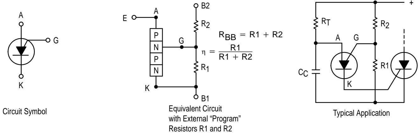
FIGURE 8 PROGRAMMABLE UNIJUNCTION
