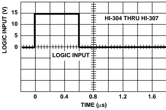
FIGURE 7C. V_{IN(LOGIC)} vs TIME
