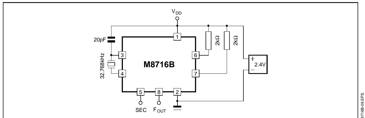
Figure 6 : Typical Application
