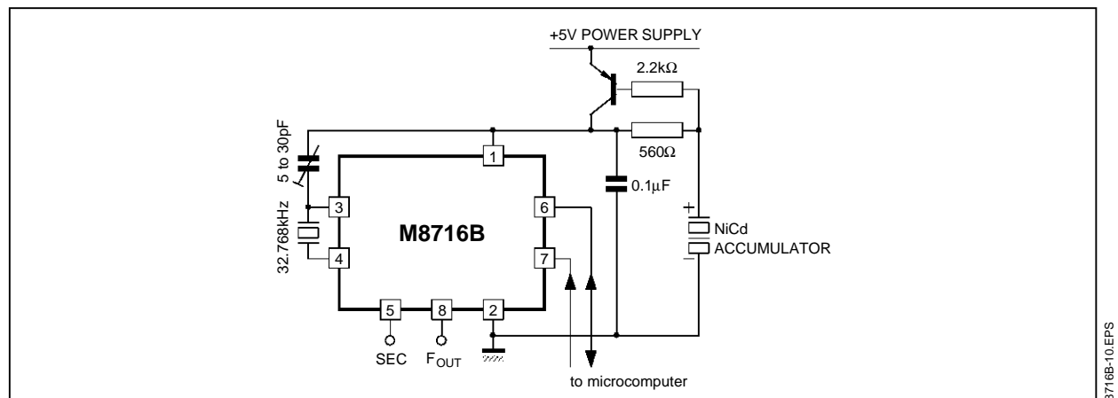
Figure 6 : Typical Application
