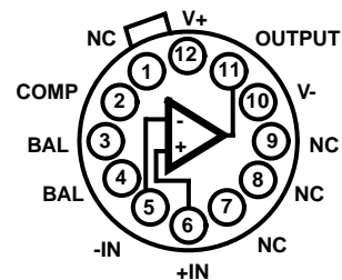
HA-2542 (METAL CAN) TOP VIEW
