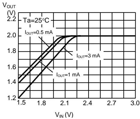
1.5 S-81230SG series
