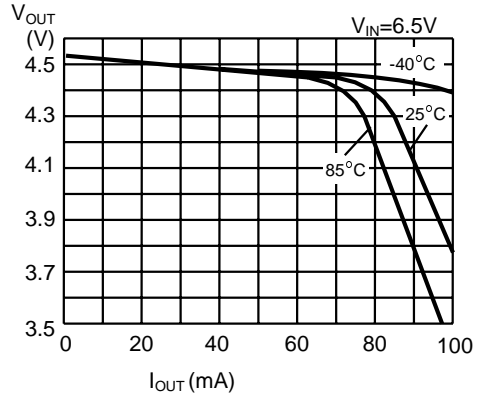
2.8 S-81245SG series
