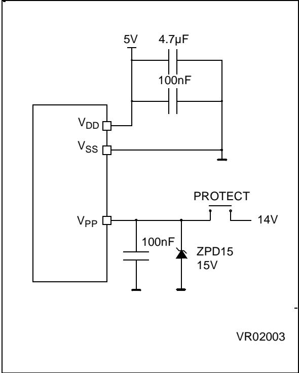
Figure 81. Programming Circuit
