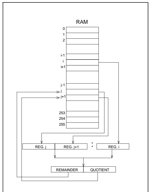
Figure 2.13 Division
