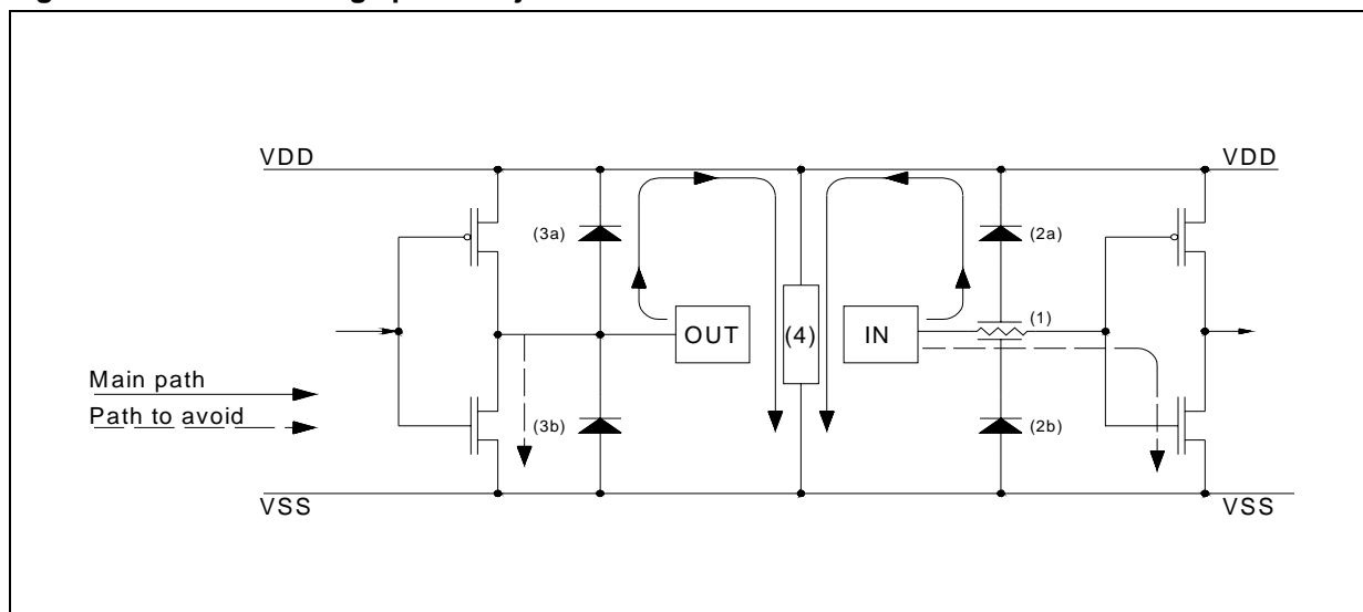
Figure 11.8 Safe discharge path subjected to ESD stress
