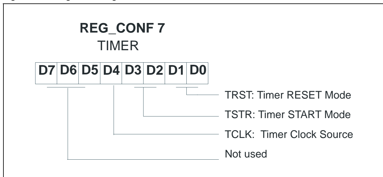
Figure 9.7 Configuration Register 7
