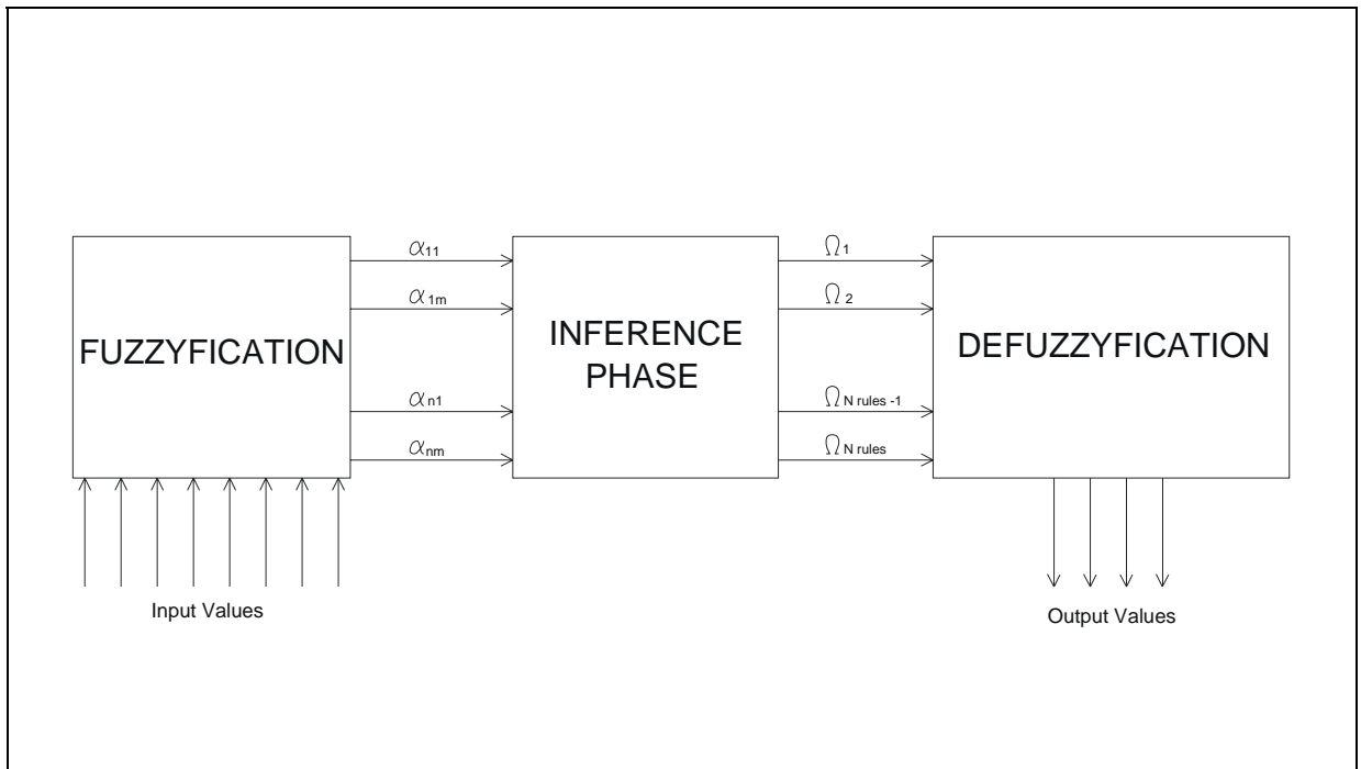
Figure 2.7 Fuzzy Inference
