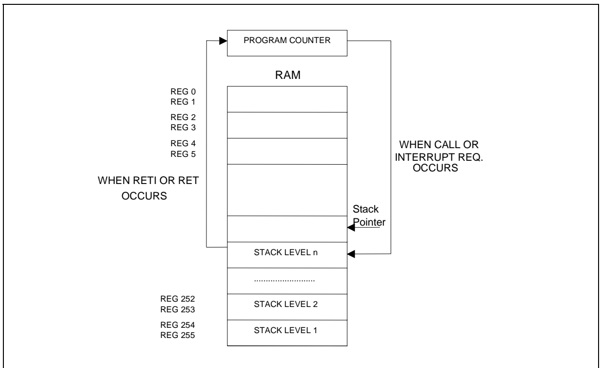
Figure 2.5 Stack Operation
