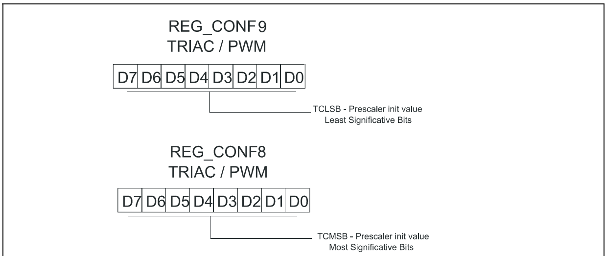
Figure 10.2 TRIAC/PWM Configuration Registers 8 and 9
