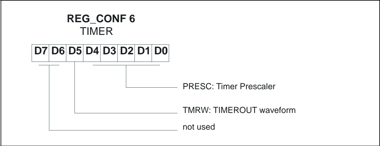
Figure 9.6 Configuration Register 6
