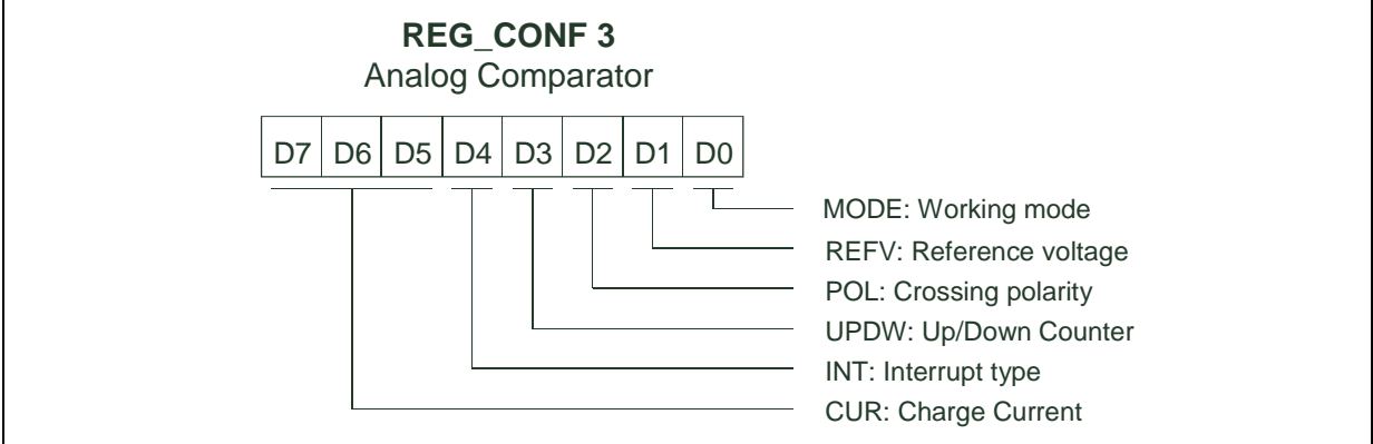
Figure 7.4 Configuration Register 15
