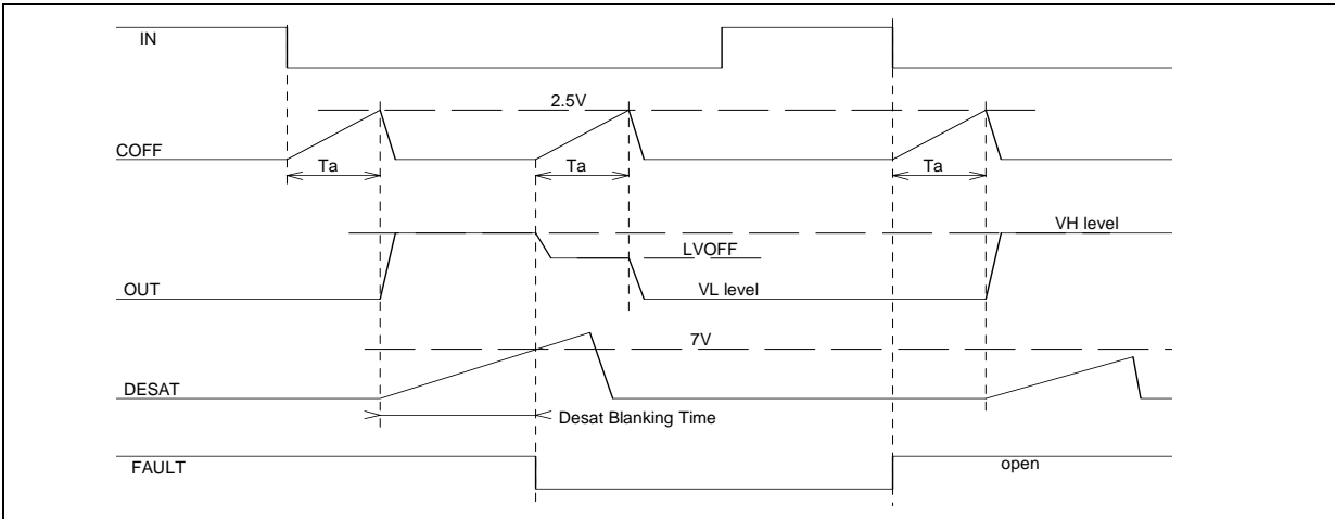
Figure 5: Desaturation fault
