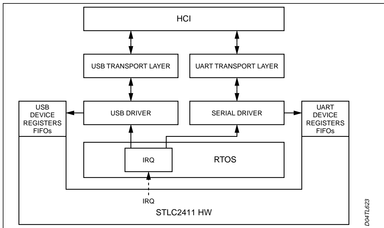
Figure 8. USB Interface
