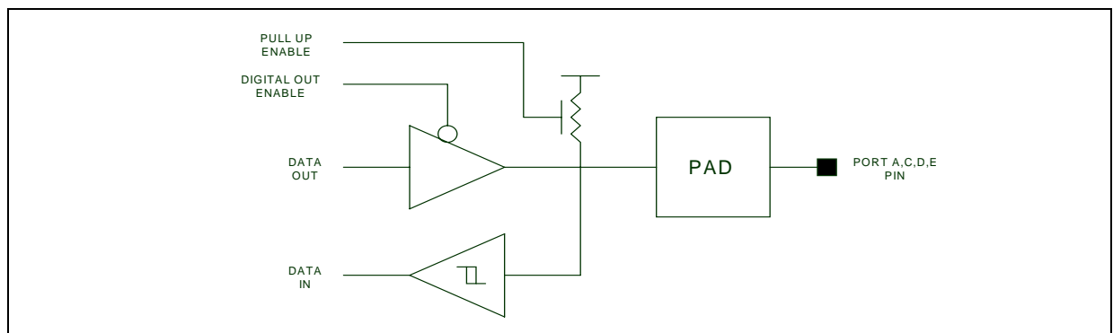
Figure 7.1 Digital Pin
