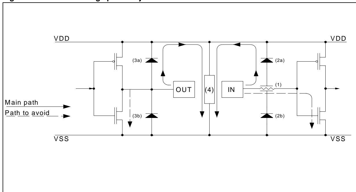
Figure 14.11 Safe discharge path subjected to ESD stress
