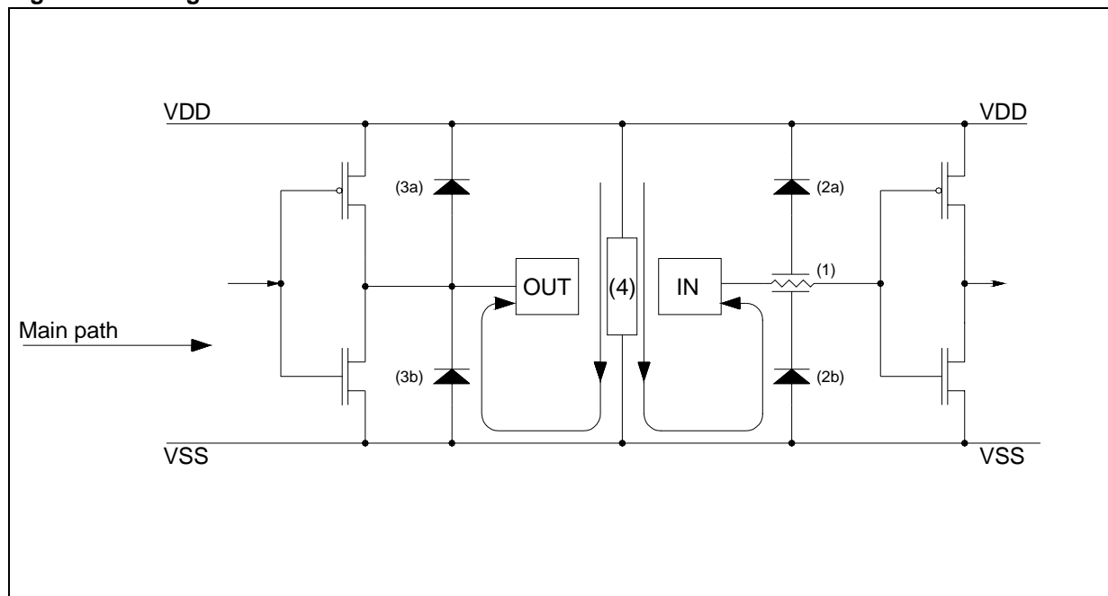
Figure 14.12 Negative Stress on a Standard Pad vs. VDD
