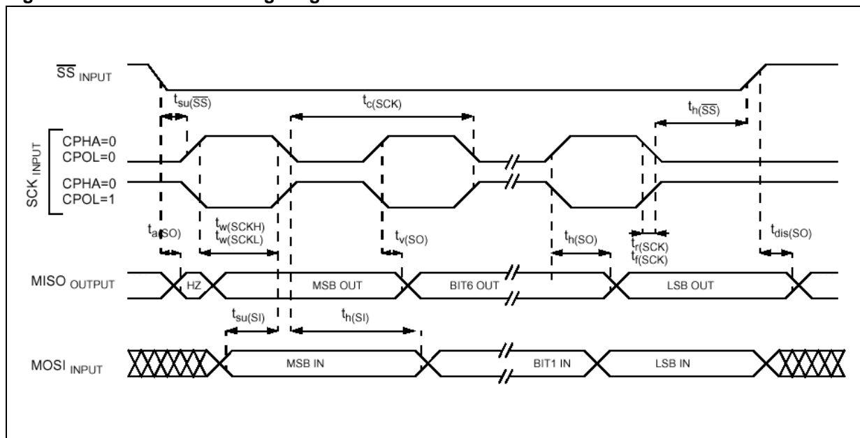
Figure 14.15 SPI Slave Timing Diagram with \text{CPHA} = 0 3)
