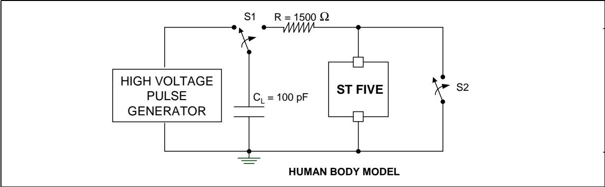
Figure 14.9 Typical Equivalent ESD Circuits
