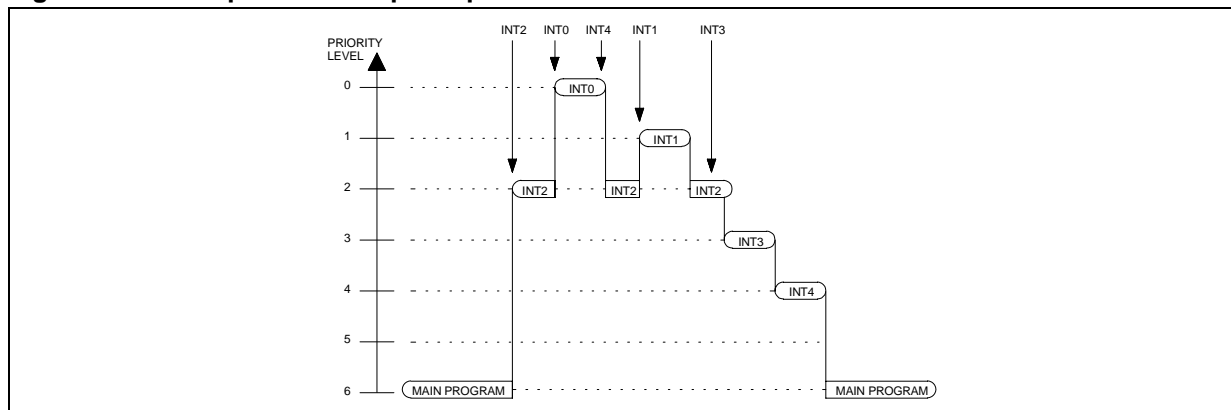
Figure 5.3 Example of Interrupt Requests
