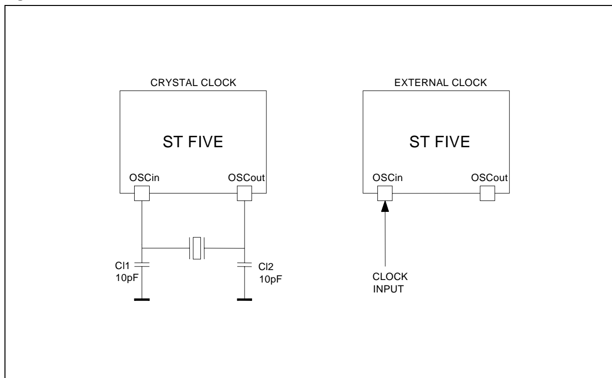
Figure 6.1 Oscillator Connections
