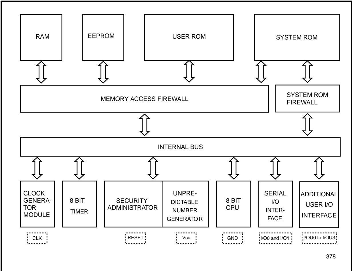
Figure 2. Block diagram
