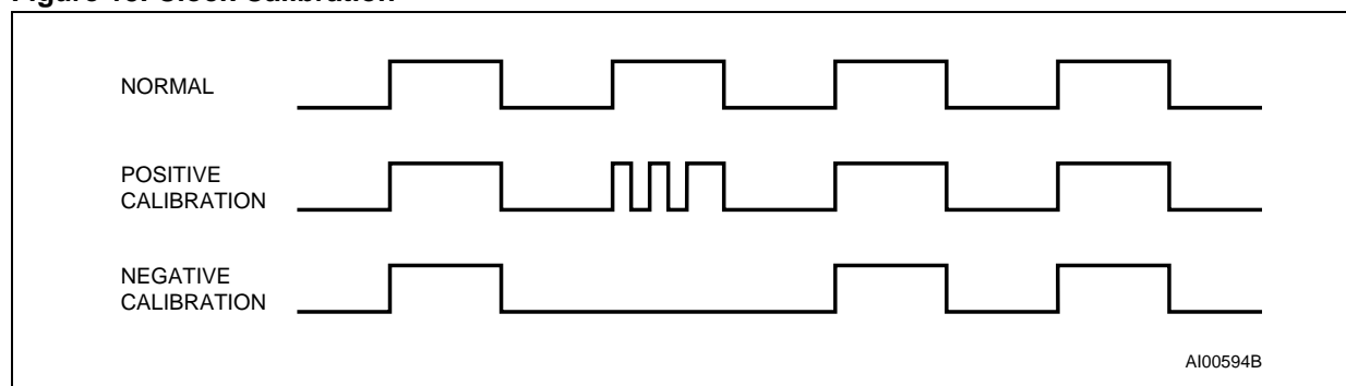
Figure 15. Clock Calibration
