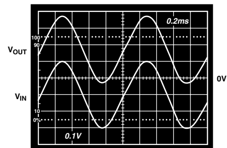
Figure 3. Input and Output Signals with V_{CM} < 0\text{ V}
