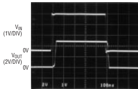
V_{IN} (1V/DIV) V_{OUT} (2V/DIV) V_S = 5V, 0V A_V = +2 100ns/DIV 1809 G44
