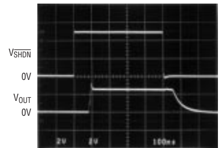
V_{SHDN} V_{OUT} V_S = 5V, 0V A_V = +2 R_L = 100\Omega 100ns/DIV 1809 G44
