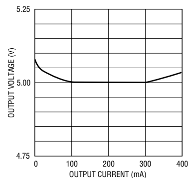
Load Regulation
