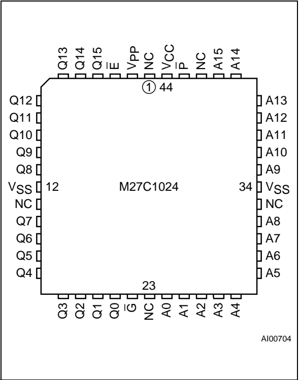
Figure 3. LCC Connections
