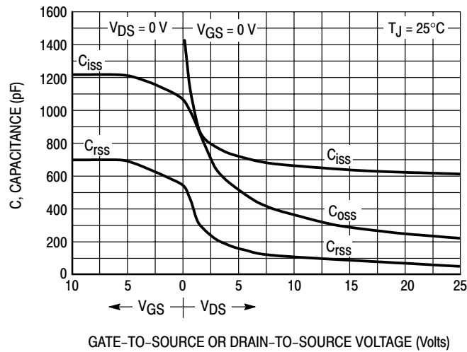
Figure 6. Capacitance Variation
