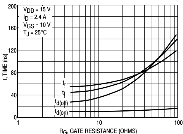
Figure 11. Resistive Switching Time Variation versus Gate Resistance
