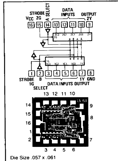
PIN-OUT DIAGRAM
