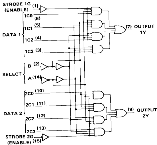
LOGIC DIAGRAM
