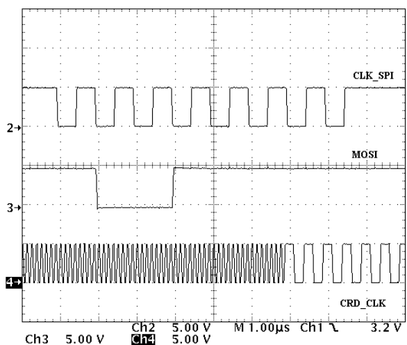
Figure 28. CRD_CLK Programming
