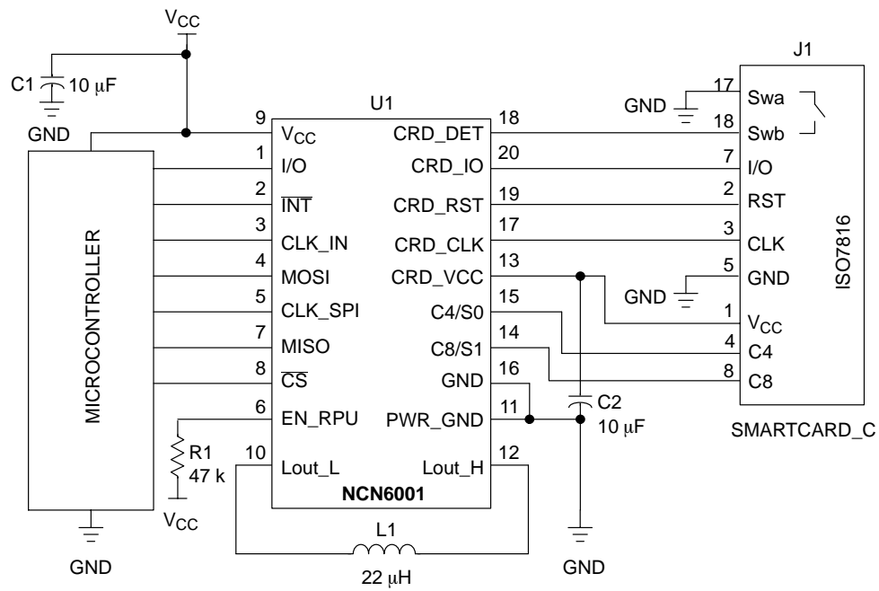
Figure 1. Typical Application
