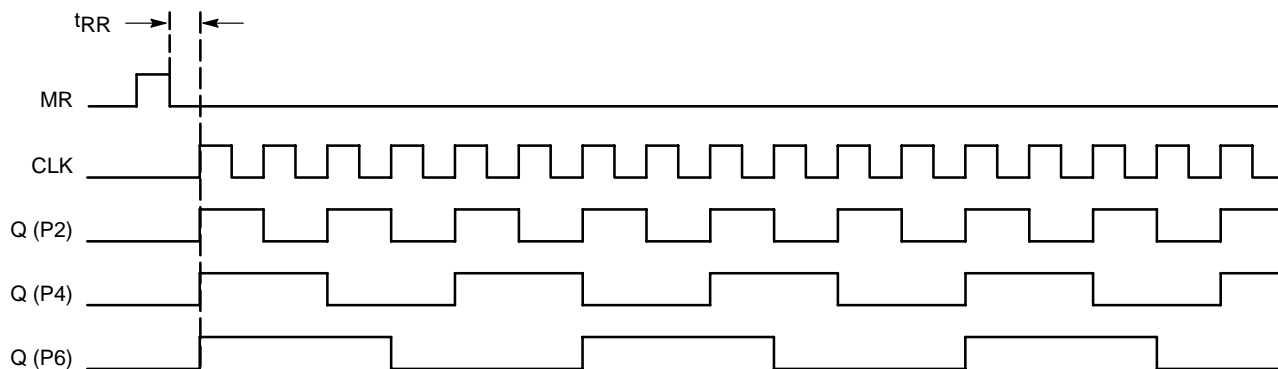
Figure 3. Timing Diagram
