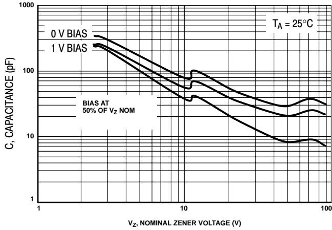
Figure 5. Typical Capacitance
