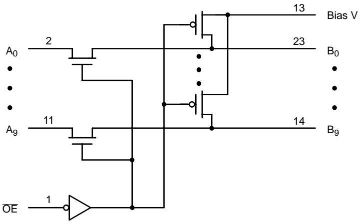
Figure 2. Logic Diagram
