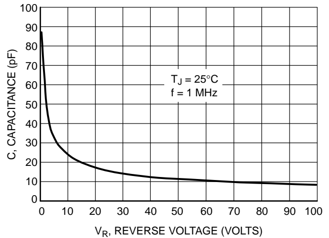
Figure 4. Typical Capacitance
